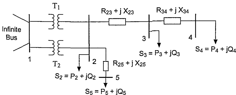
Figure 7.27 The Feeder of Problem 7.14.
