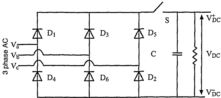
Figure 3.54 A Three-Phase Rectifier.
