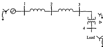
Figure 8.48 The System for Example 8.6
