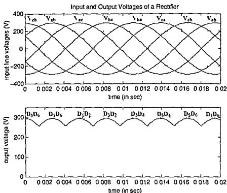
Figure 3.55 The Input Line to Line Voltage and the Output Voltage of a Three-Phase Rectifier with the Switches Conducting Shown
