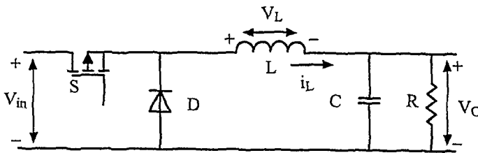
Figure 3.40 A Buck Converter Circuit.
