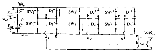
(f) V_{an} = V_{cn} = V_{idc} , V_{bn} = 0 , I_a, I_b < 0 , I_c > 0 , D_1^+ on, SW_2^- on, SW_3^+ on
