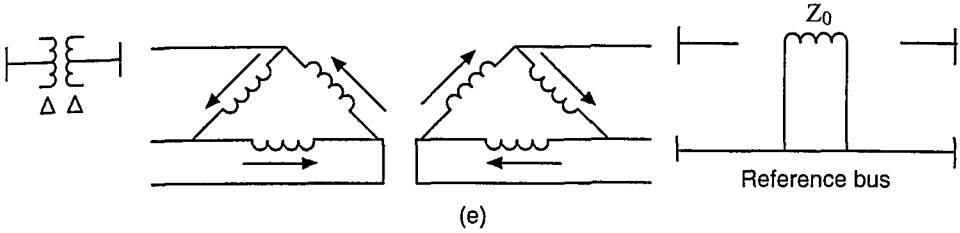
Figure 8.18 Zero-Sequence Equivalent Circuits of Three-Phase (a) Y-Y-Connected Transformer Banks with One Side Grounded, (b) Y-Y-Connected Transformer Banks with Both Sides Grounded, (c) Grounded Y-Δ-Connected Transformer Banks, (d) Ungrounded Y-Δ-Connected Transformer Banks, and (e) Δ-Δ-Connected Transformer Banks.
