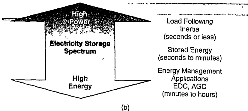
Figure 4.15 (b) The Energy Management Time Scale of Power Grid Control. 12
