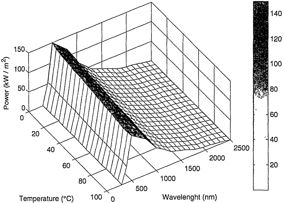
Figure 5.16 Spectra for Photovoltaic Performance Evaluation. 12,15
