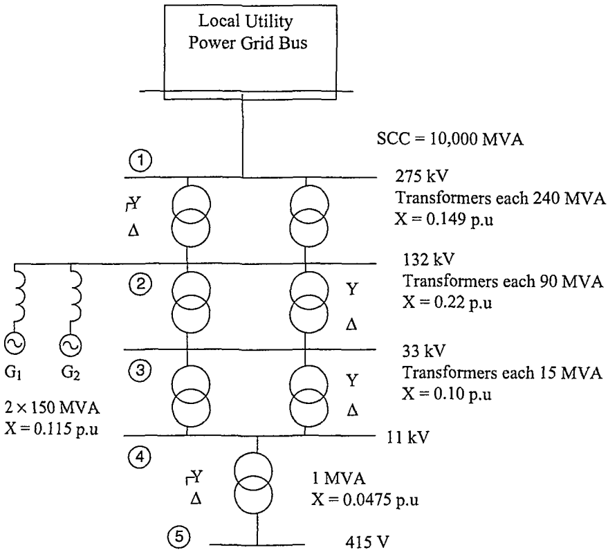
Figure 8.38 A One-Line Diagram of Example 8.4.
