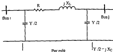
Figure 8.36 The Equivalent Impedance of the Transmission Line Model for Example 8.3
