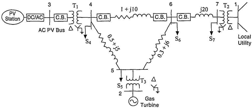
Figure 4.44 One-Line Diagram for Example 4.7.
