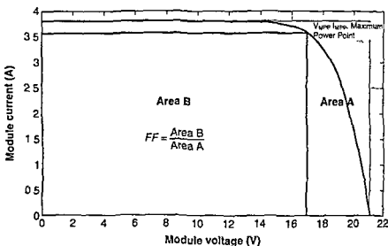
Figure 5.9 Photovoltaic Module Fill Factor
