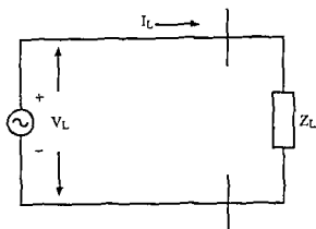
Figure 2.22 The Inductive Impedance Load Model
