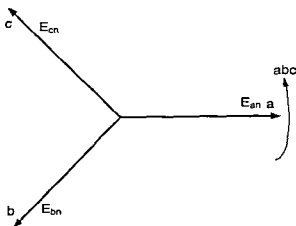
Figure 2.16 A Balanced Three Phase System
