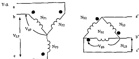
Figure 2.52 A Three-Phase Y-Δ Connection
