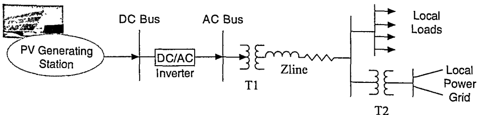
Figure 3.66 A One-Line Diagram for Problem 3.1.
