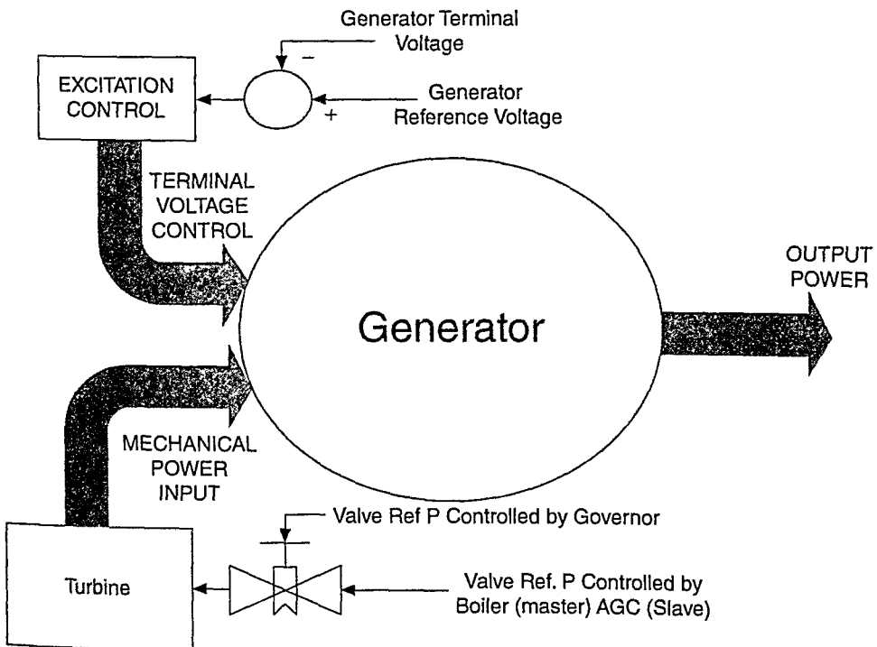
Figure 4.13 A Generator as a Three-Terminal Device.
