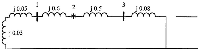
Zero Sequence
