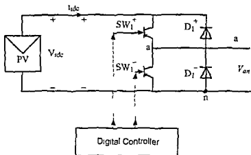
Figure 3.3 A Single Phase DC/AC Inverter with Two Switches
