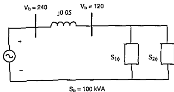
Figure 2.51 The Per Unit Equivalent of Fig 2.48
