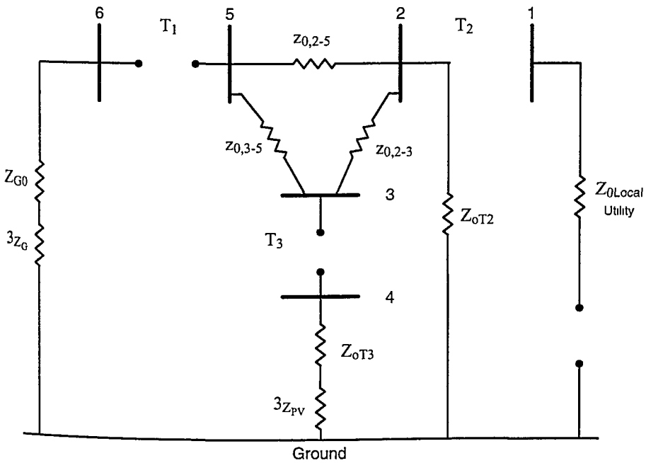
Figure 8.21 The Zero Sequence Network of Fig. 8.20.
