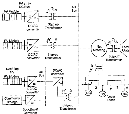
Figure 3.27 One-Line Diagram for a Community Microgrid Distribution System Connected to a Local Utility Power Grid
