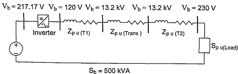
Figure 3.29 The Per Unit Model of Fig. 3.28.
