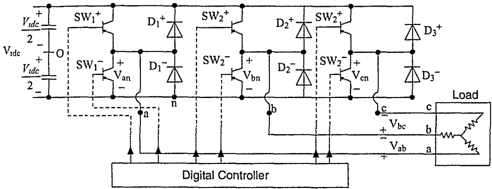
Figure 3.20 Three-Phase Inverter Topology.
