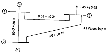
Figure 7.33 The System for Problem 7.20
