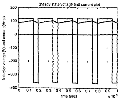
Figure 3.39 Inductor Voltage and Current for Example 3.10
