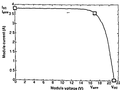
Figure 5.8 The Operating Characteristics of a Photovoltaic Module 9
