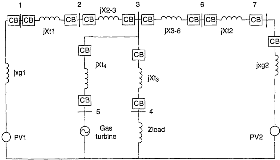
Figure 4.43 The Impedance Diagram of Figure 4.42.
