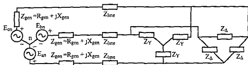
Figure 2.19 A Three Phase System with Two Loads
