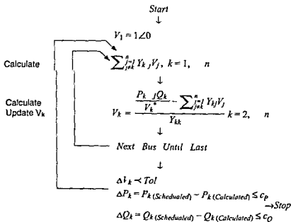
Figure 7.13 The Gauss-Seidel Algorithm for Iterative Approximation
