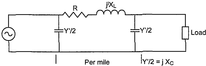
Figure 7.22 The Transmission-Line Pie Model.
