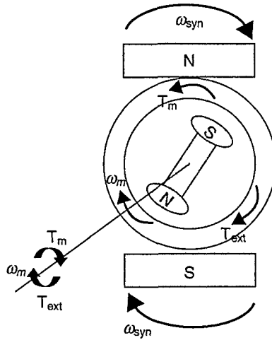
Figure 6.28 The Operation of an Induction Machine as a Generator.
