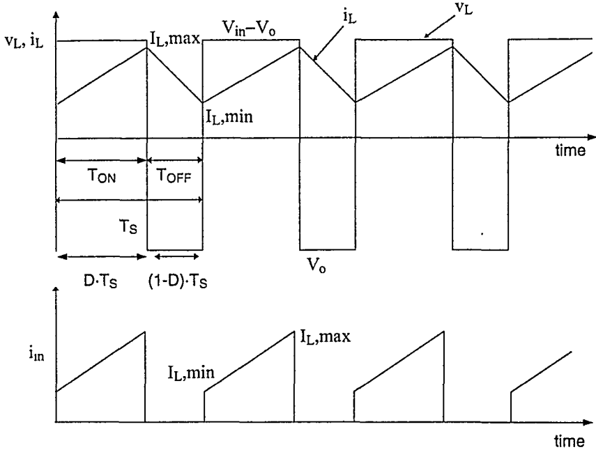
Figure 3.53 The Input Current Waveform of a Buck-Boost Converter.
