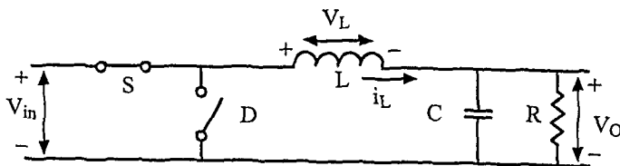
Figure 3.41 The Equivalent Circuit of a Step-Down Converter When the Switch S Is Closed.
