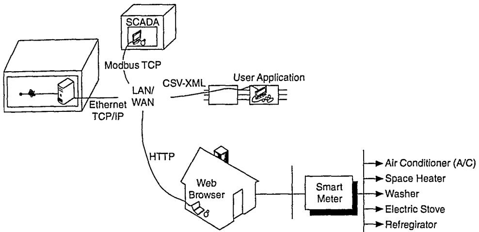
Figure 4.25 Ethernet TCP/IP Sensors, Transducers, and Communication Protocol for Load Control.
