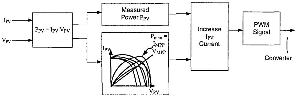
Figure 5.27 A Maximum Power Point Tracking Control Algorithm.
