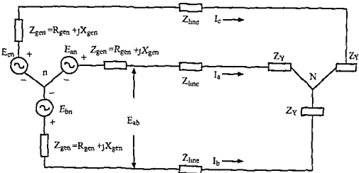
Figure 2.13 A Balanced Three-Phase System
