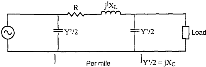
Figure 4.50 A Transmission Line Pie Model.
