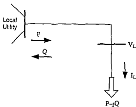
Figure 2.27 The Power Model for a Capacitive Load
