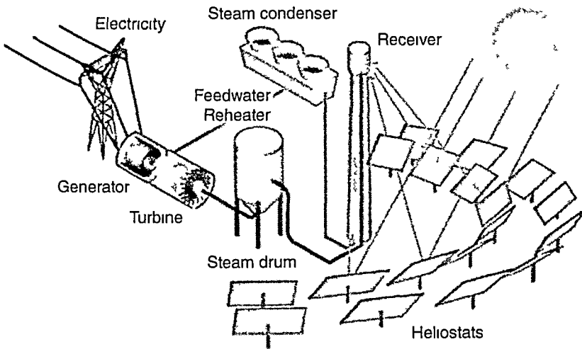
Figure 5.4 A Steam Solar Power Generating Station. 1
