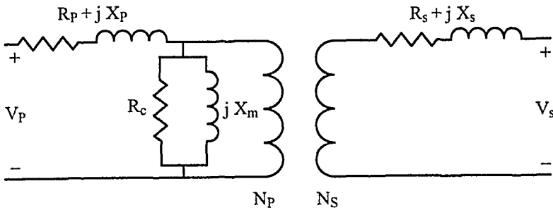
Figure 2.37 The Complete Schematic of a Real Transformer.
