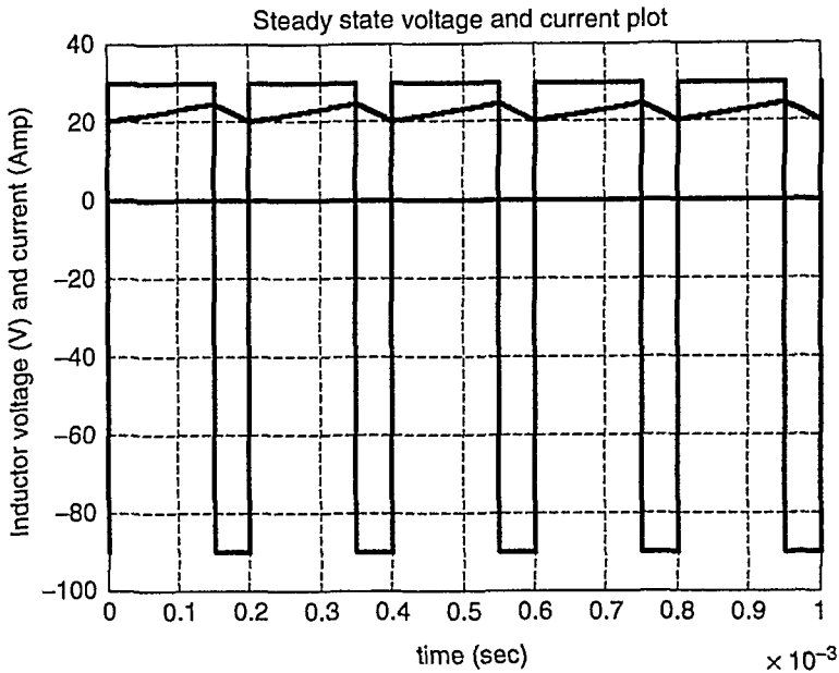
Figure 3.46 The Inductor Voltage and Current for Example 3.12.
