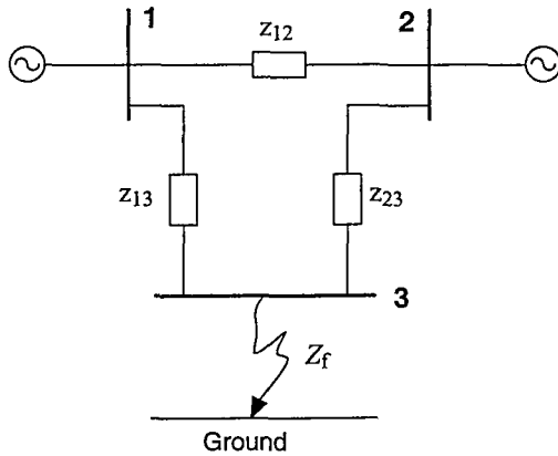
Figure 8.33 A Fault at Bus 3.
