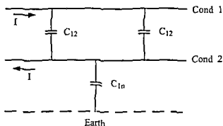
Figure 2.57 Capacitance between Two Conductors and Ground
