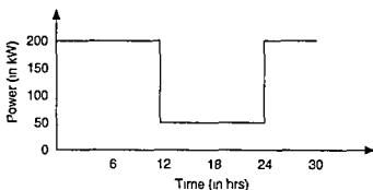
Figure 4.22 The Load for 24 Hours for Example 4.2
