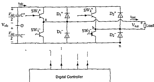
Figure 3.12 A Single Phase DC/AC Converter with Four Switches.
