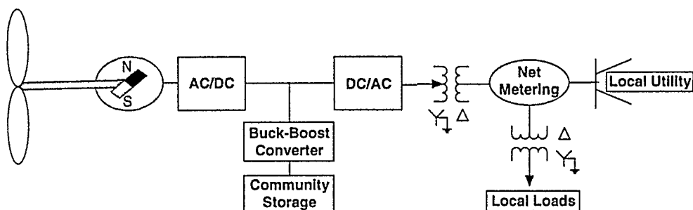
Figure 3.1 A Variable-Speed Permanent Magnet Wind Generator System. 1
