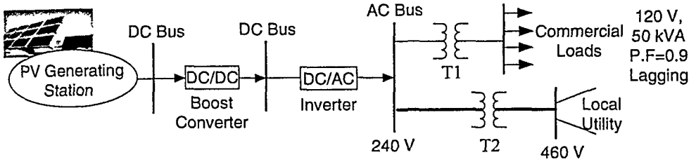
Figure 3.37 One-Line Diagram of Example 3.9.
