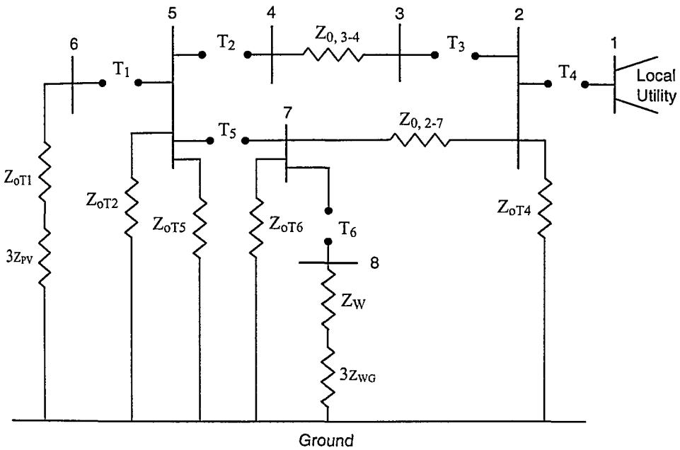
Figure 8.23 The Zero Sequence Network of Fig. 8.22.
