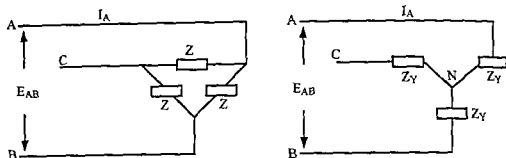
Figure 2.18 \Delta Connected Loads and Equivalent Y Connected Loads
