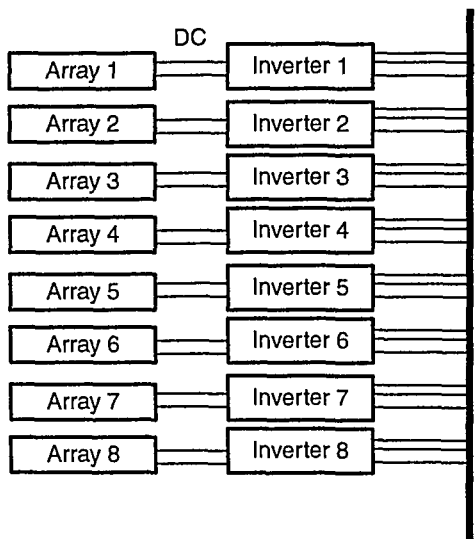
Figure 5.14 General Structure of Photovoltaic Arrays with Inverters.
