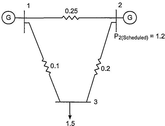
Figure 7.14 The One-Line Diagram of Example 7.4.
