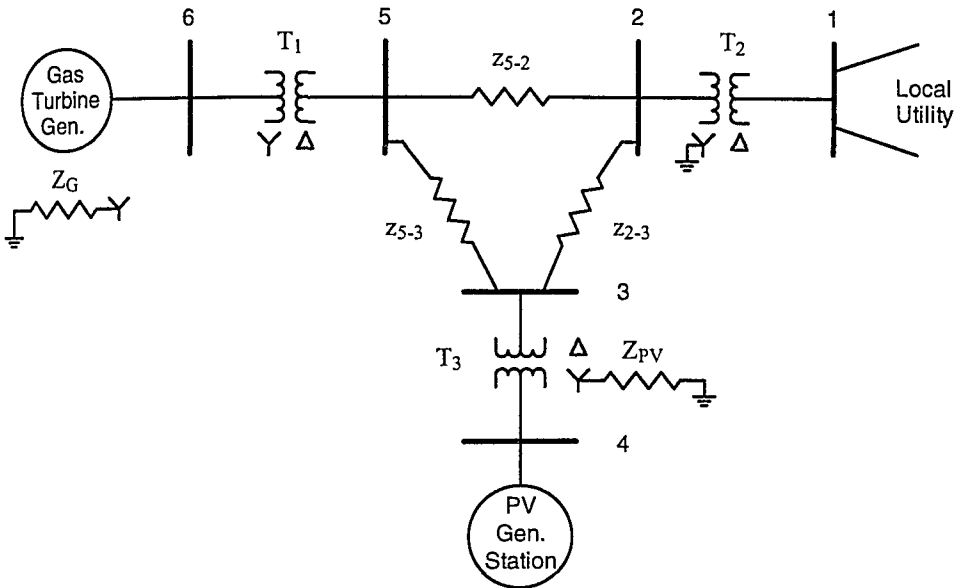
Figure 8.20 A Balanced Three-Phase Microgrid.
