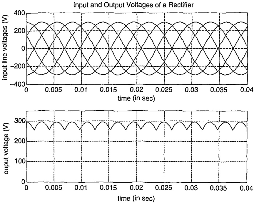
Figure 3.56 The Result of the Simulation.
