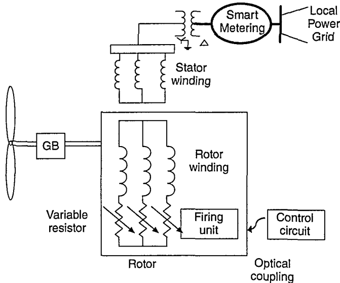
Figure 6.35 A Microgrid of an Induction Machine Controlled as an Induction Generator Supplying Power to the Local Power Grid.
