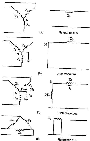
Figure 8 19 Zero Sequence Equivalent Circuit (a) for a Y Connected Ungrounded Load (b) for a Grounded Y Connected Load (c) for a Y Connected Load with Grounding Impedance and (d) for a Δ Connected Load
