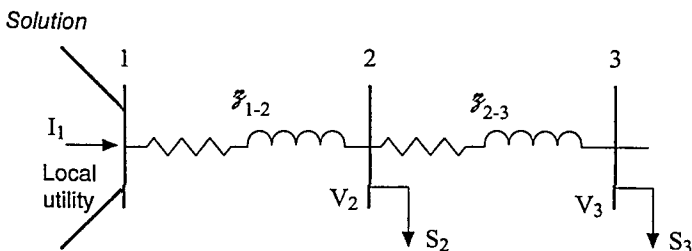
Figure 7.1 The One-Line Diagram of Example 7.1.
