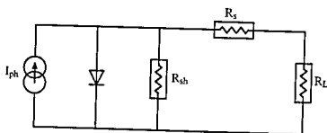
Figure 5.24 A Photovoltaic Model and Its Load
