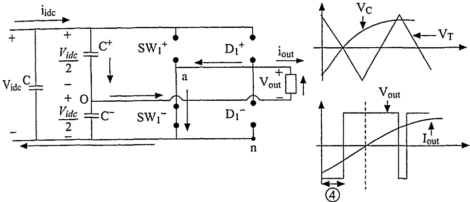
Figure 3.10 (a-d) The Equivalent Circuit of the Single-Phase Inverter with Two Switches for Various Operating Conditions.
