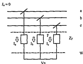
Figure 8.2 A Balanced Three-Phase Fault
