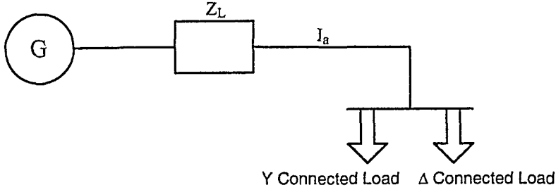
Figure 2.20 A One-Line Diagram of Fig. 2.19.
