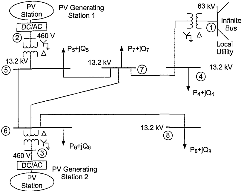
Figure 7.21 The Photovoltaic Microgrid of Example 7.7.
