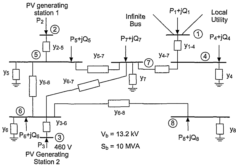
Figure 7.20 A One-Line Injection Model of a Microgrid.
