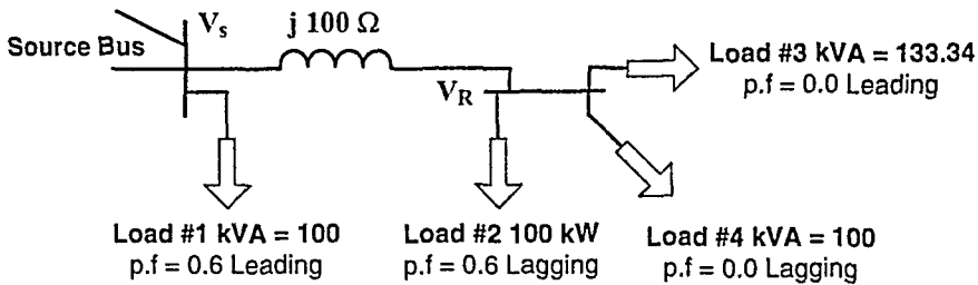
Figure 2.67 The One-Line Diagram of Problem 2.17.
