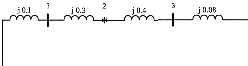
Negative Sequence
