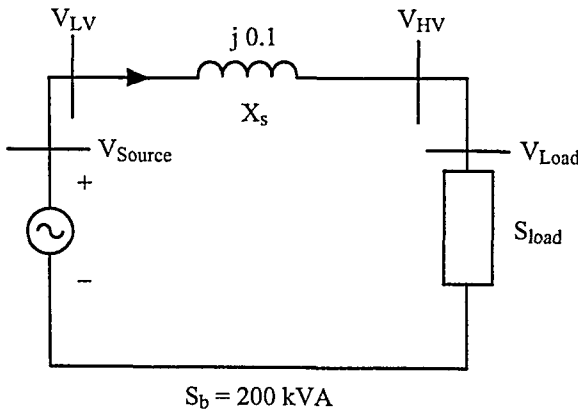
Figure 2.47 Per Unit Equivalent Circuit of Example 2.9.
