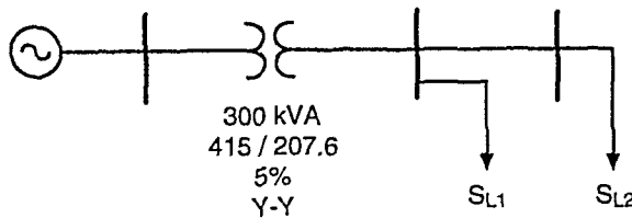
Figure 2.49 One-Line Diagram of Fig. 2.48.
