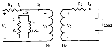
Figure 2.36 The Schematic of a Real Transformer
