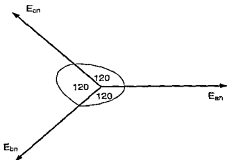
Figure 2.10 The Balanced Three Phase System
