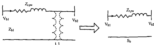
Figure 2.46 The Per Unit Equivalent Circuit of Fig 2.45
