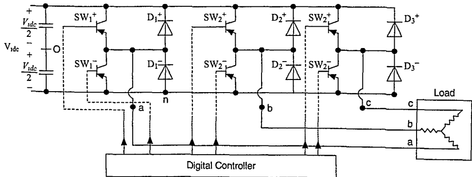
Figure 3.69 The Linear and Overmodulated Operation of a Three-Phase Converter.
