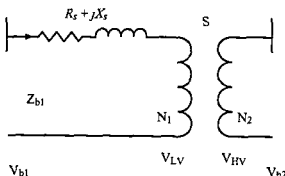
Figure 2.45 The Equivalent Circuit of a Transformer
