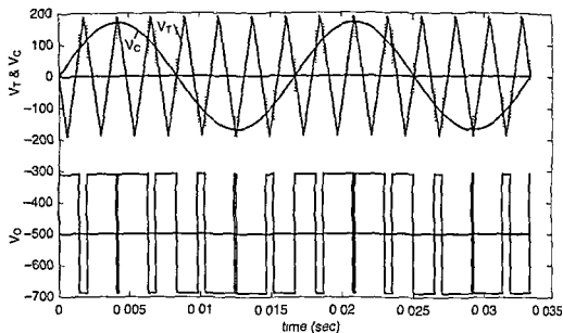
Figure 3.19 Plot of V_T(t) and V_C(t) and V_o for Example 3.3 Using the Equation of Line of Triangular Method
