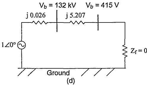
Figure 8.40 (a-d) The Impedance Diagram of Example 8.4, Part ii.
