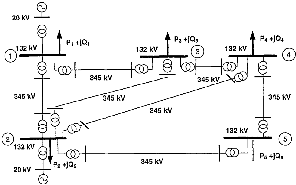
Figure 2.3 A Five-Bus Bulk Power Grid.
