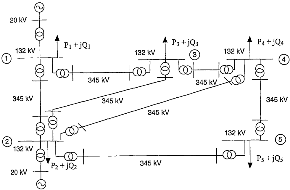
Figure 4.2 A Five-Bus Power System.
