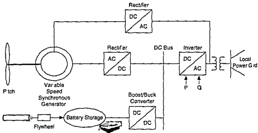
Figure 6 42 A Microgrid of a Multipole Synchronous Generator
