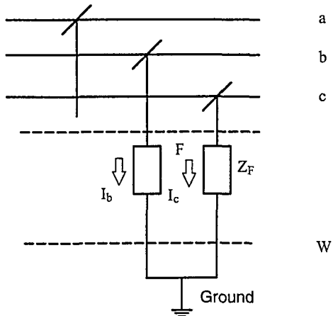
Figure 8.4 An Unbalanced Fault: Two Lines to Ground.
