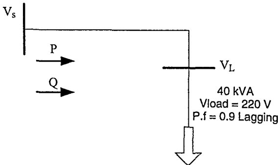
Figure 2.28 The Power Model for Example 2.4.
