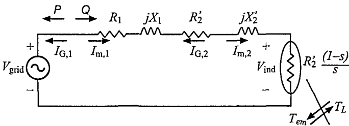
Figure 6.30 The Single-Phase Equivalent Circuit of Induction Generator.
