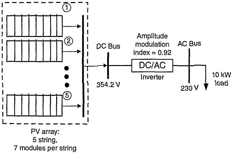
Figure 5.17 The One-Line Diagram of Example 5.1.
