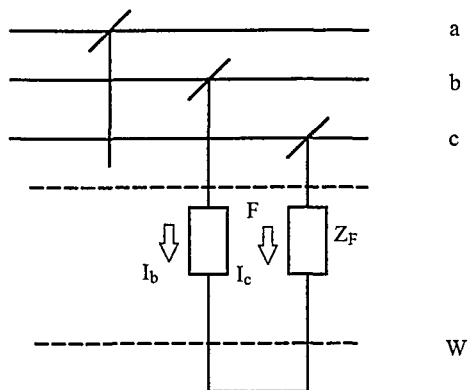
Figure 8.5 An Unbalanced Fault: Line to Line.
