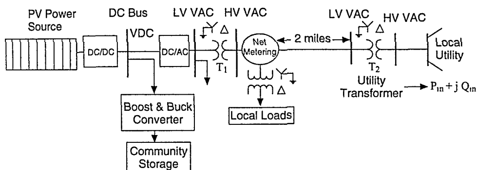
Figure 3.2 A Radial Photovoltaic Microgrid Distributed Generation System. 1
