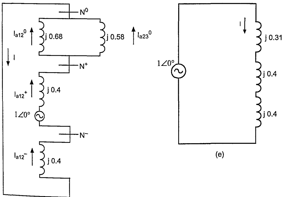
Figure 8.49 For Example 8.6, part i: (a) Zero Sequence Network, (b) Positive Sequence Network, (c) Negative Sequence Network, (d) Connection Diagram for Single Line to Ground Fault at Bus 2, and (e) Simplified Circuit of (d).
