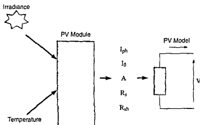
Figure 5.20 The Modeling of a Photovoltaic Module
