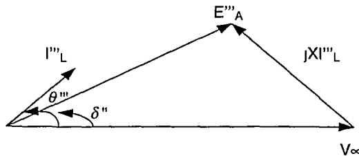
Figure 4.40 The Phasor Diagram of a Generator Operating with a Leading Power Factor.
