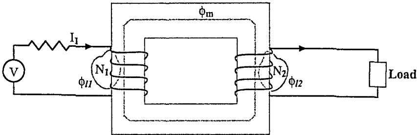
Figure 2.34 An Ideal Single-Phase Transformer.
