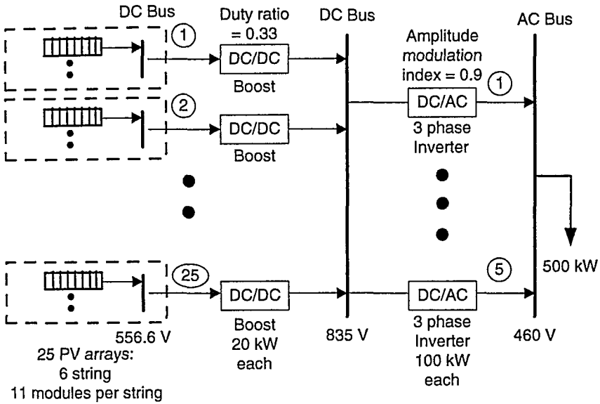
Figure 5.18 The One-Line Diagram of Example 5.2.
