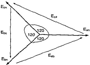
Figure 2.14 Phase Voltages and Line-Line Voltages
