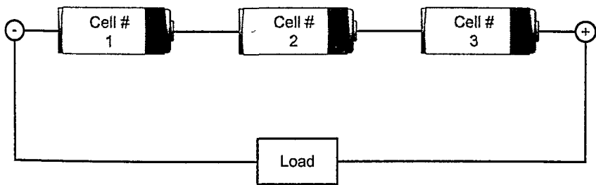
Figure 5.33 Three Single Cells in a String.
