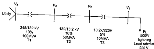
Figure 7.34 The System for Problem 7.21
