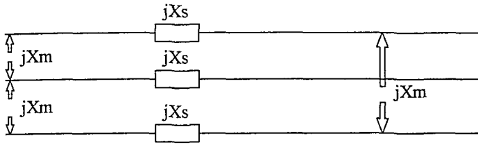
Figure 8.25 The Balanced Three-Phase Transmission Line of Fig. 8.24.
