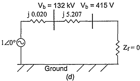
Figure 8.39 (a-d) The Impedance Diagram of Example 8.4.
