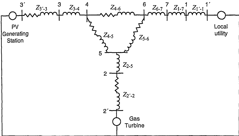
Figure 4.46 Model for Short-Circuit Studies.
