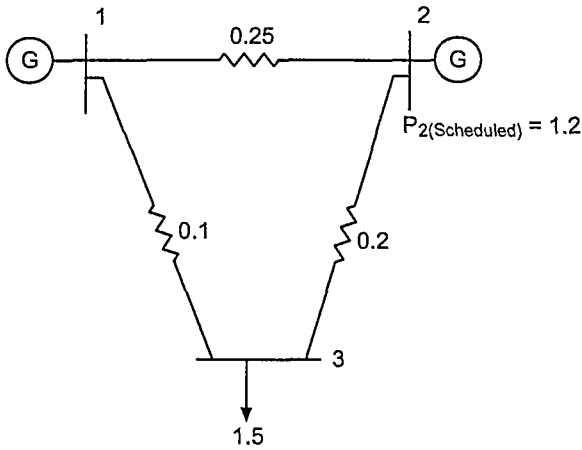
Figure 7.19 The One-Line Diagram of Example 7.6.
