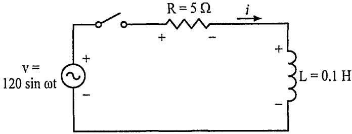
Figure 2.5 An R-L Circuit.
