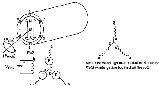
Figure 4.30 A Three Phase Synchronous Generator
