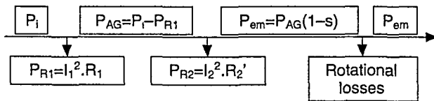
Figure 6.19 The Power Flow in Induction Machines.
