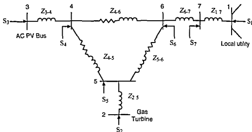
Figure 4.45 Model for Power Flow Studies.
