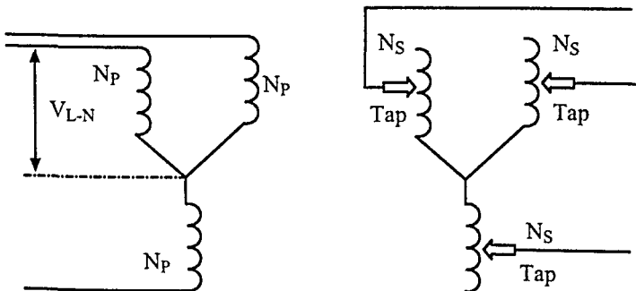
Figure 2.54 A Schematic of a Three-Phase Y-Y Connected Tap Changing Transformer.
