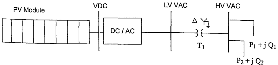
Figure 3.23 A Microgrid Stand-Alone Photovoltaic System.
