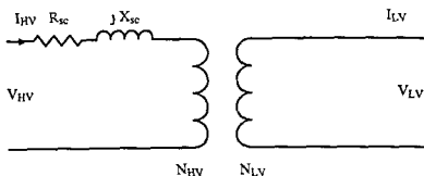
Figure 2.39 The Equivalent Model of a Transformer
