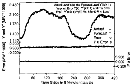
Figure 4.3 A 24 Hour Load Variation Sampled Every 5 Minutes. 7
