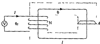
Figure 6.8 An Inductor Winding
