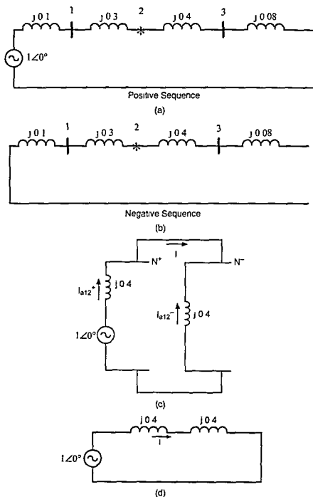
Figure 8.52 For Example 8.7: (a) Positive Sequence Network, (b) Negative Sequence Network, (c) Connection Diagram for Double Line Fault at Bus 2 and (d) the Simplified Circuit of (c)
