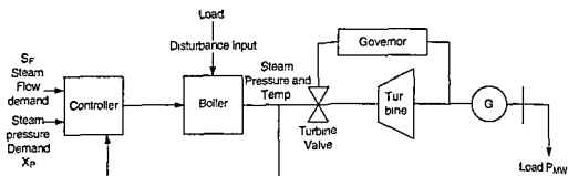
Figure 4 11 A Boiler Control System 11
