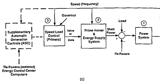
Figure 4 15(c) The Automatic Generation Control (AGC) Block Diagram
