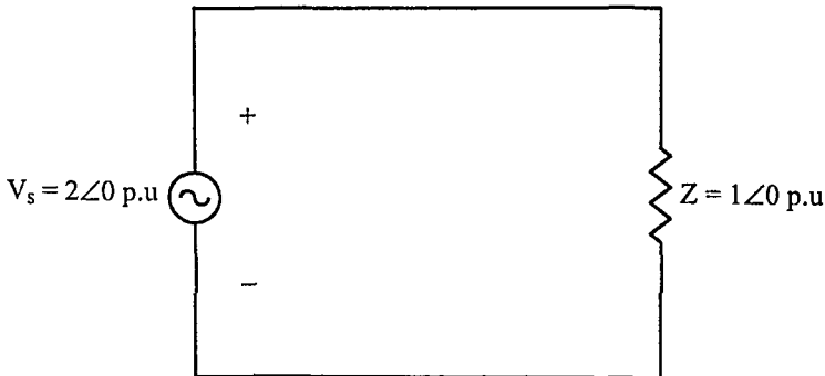
Figure 2.43 The Per Unit Equivalent Circuit of Example 2.8.
