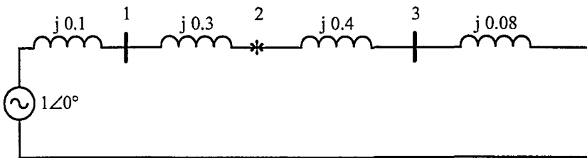
Positive Sequence
