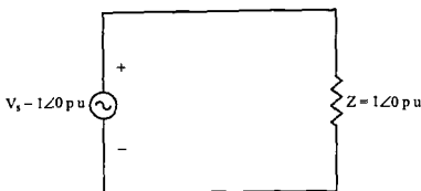
Figure 2.42 The Equivalent Circuit of Example 2.7
