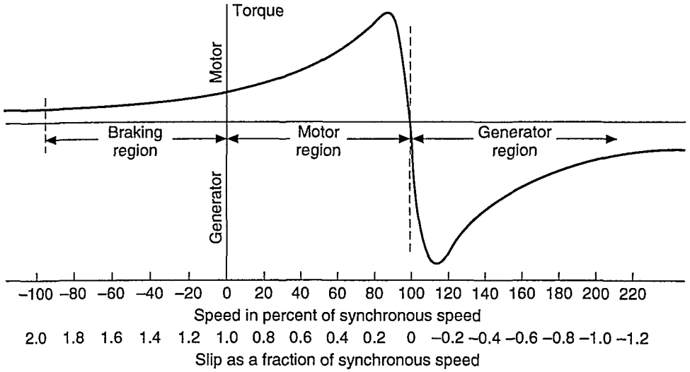
Figure 6.21 An Induction Machine's Various Regions of Operation.
