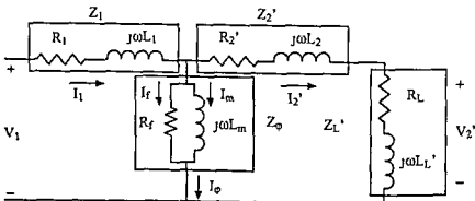
Figure 2 65 Equivalent Circuit for Problem 2 3
