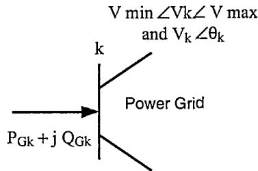
Figure 7.8 A Photovoltaic or Wind Generating Bus Model.
