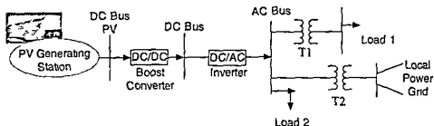
Figure 3.67 A One Line Diagram of Problem 3.2
