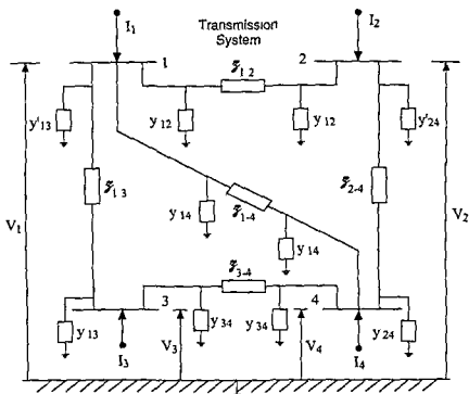
Figure 7.10 A Current Injection Model for Power Flow Studies
