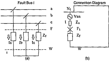
Figure 8.32 The Balanced Three Phase (a) Fault and (b) the Thevenin Equivalent Circuit
