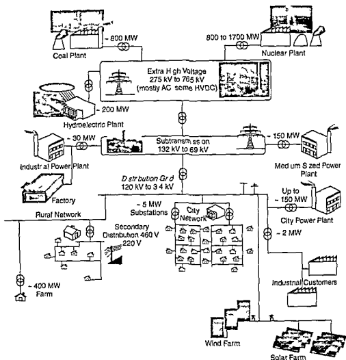
Figure 2.2 A Power System Interconnected Network with High Green Energy Penetration 6
