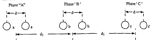
Figure 2 59 Three Phase Transmission Line with Bundled Conductor Lines
