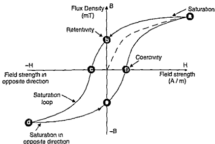
Figure 6.9 A Schematic of a Hysteresis Loop 19
