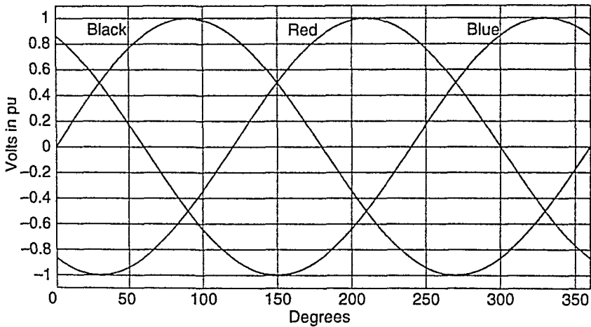
Figure 2.4 Three-Phase Generator Voltage Wave Forms. 7
