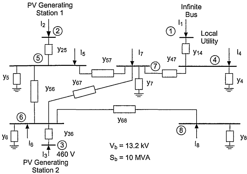
Figure 7.23 The Current Injection Model of Example 7.7.
