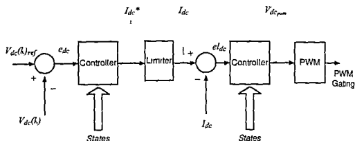
Figure 3.57 The Control Diagram of DC Bus Voltage Regulation Using a Rectifier System
