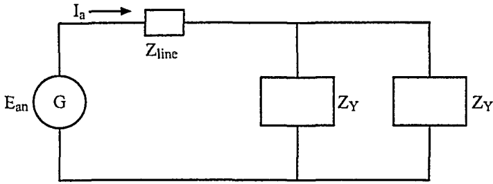
Figure 2.21 One-Phase Equivalent Circuit of Fig. 2.19.
