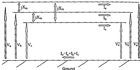
Figure 8.14 A Balanced Three Phase Transmission Reactance Model
