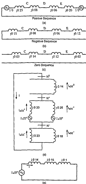
Figure 8.46 For Example 8.5: (a) Positive Sequence Network, (b) Negative Sequence Network, (c) Zero Sequence Network, (d) Connection Diagram of Sequence Networks for Single Line to Ground Fault at Bus D, and (e) Simplified Circuit of (d)
