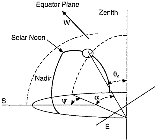
Figure C.4 Solar Noon and Equator Definition of Angles. 1
