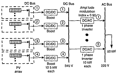
Figure 5.32 The One Line Diagram of Example 5.4
