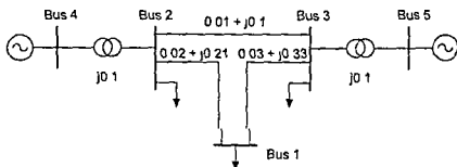
Figure 7.28 The System for Problem 7.15
