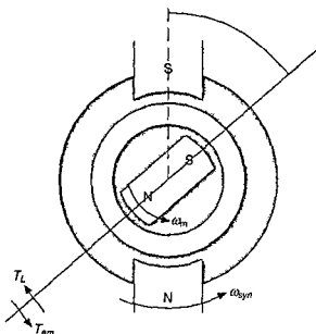
Figure 6.13 The Schematic Flux Distributions for Two Pole Machines.
