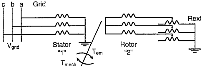
Figure 6.14 The Equivalent Circuit of a Wound Rotor Induction Machine with External Resistance, R_{ext} , Inserted in the Rotor Circuit.
