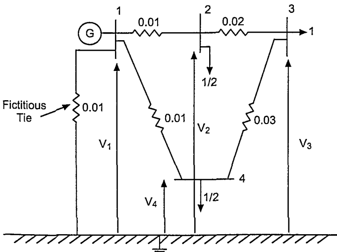
Figure 7.16 The One-Line Diagram of Example 7.5.
