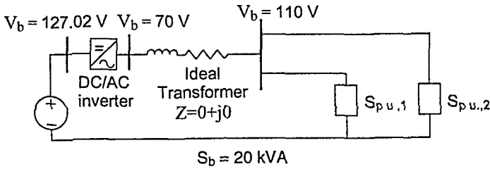
Figure 3.24 Per Unit Model of Fig. 3.23.
