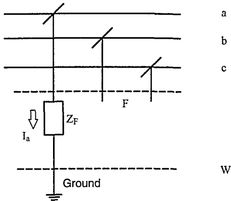
Figure 8.3 An Unbalanced Fault: One Line to Ground.
