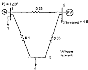
Figure 7.31 The One Line Diagram of Problem 7.18
