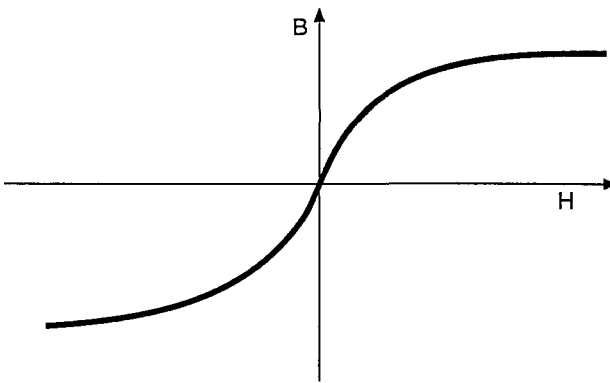
Figure 6.11 The Normalized Magnetization Curve.
