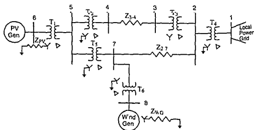
Figure 8.22 A Balanced Three Phase Wind Power Microgrid
