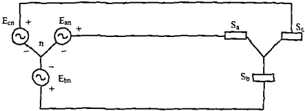
Figure 2.12 A Balanced Three-Phase Three-Wire Distribution System
