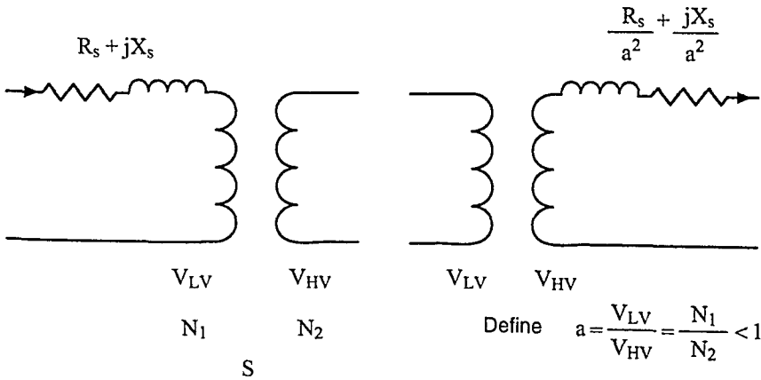
Figure 2.44 The Equivalent Circuit of a One-Phase Transformer.
