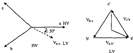
Figure 2.53 A 30° Phase Shift in Y-Δ Transformers.
