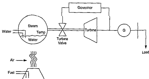
Figure 4 10 The Governor Control System 11
