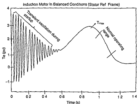
Figures 6.34 The Dynamic Performance of an Induction Machine
