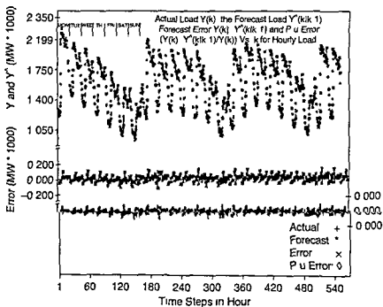
Figure 4.4 A Weekly Load Variation Sampled Hourly
