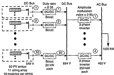
Figure 5.19 The One-Line Diagram of Example 5.3
