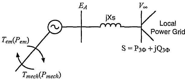
Figure 4.34 The Operation of a Generator Injecting Power into a Local Power Grid.
