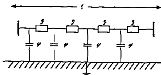
Figure 2.61 A Distributed Model of Transmission Lines
