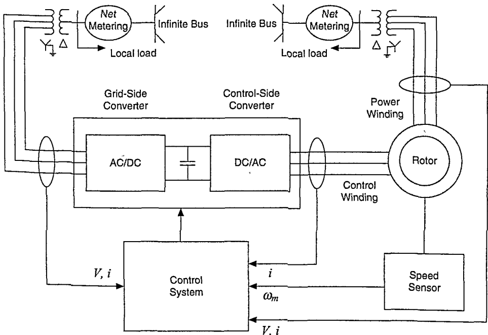
Figure 6.40 A Microgrid of Brushless Doubly-Fed Induction Generator.
