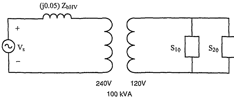
Figure 2.50 One-Phase Equivalent Circuit Model of Fig. 2.48.
