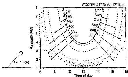
Figure C.2 Air Mass Calculated for a Specific Location 9
