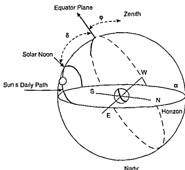
Figure C.3 Solar Noon and Definition of Angles. 9
