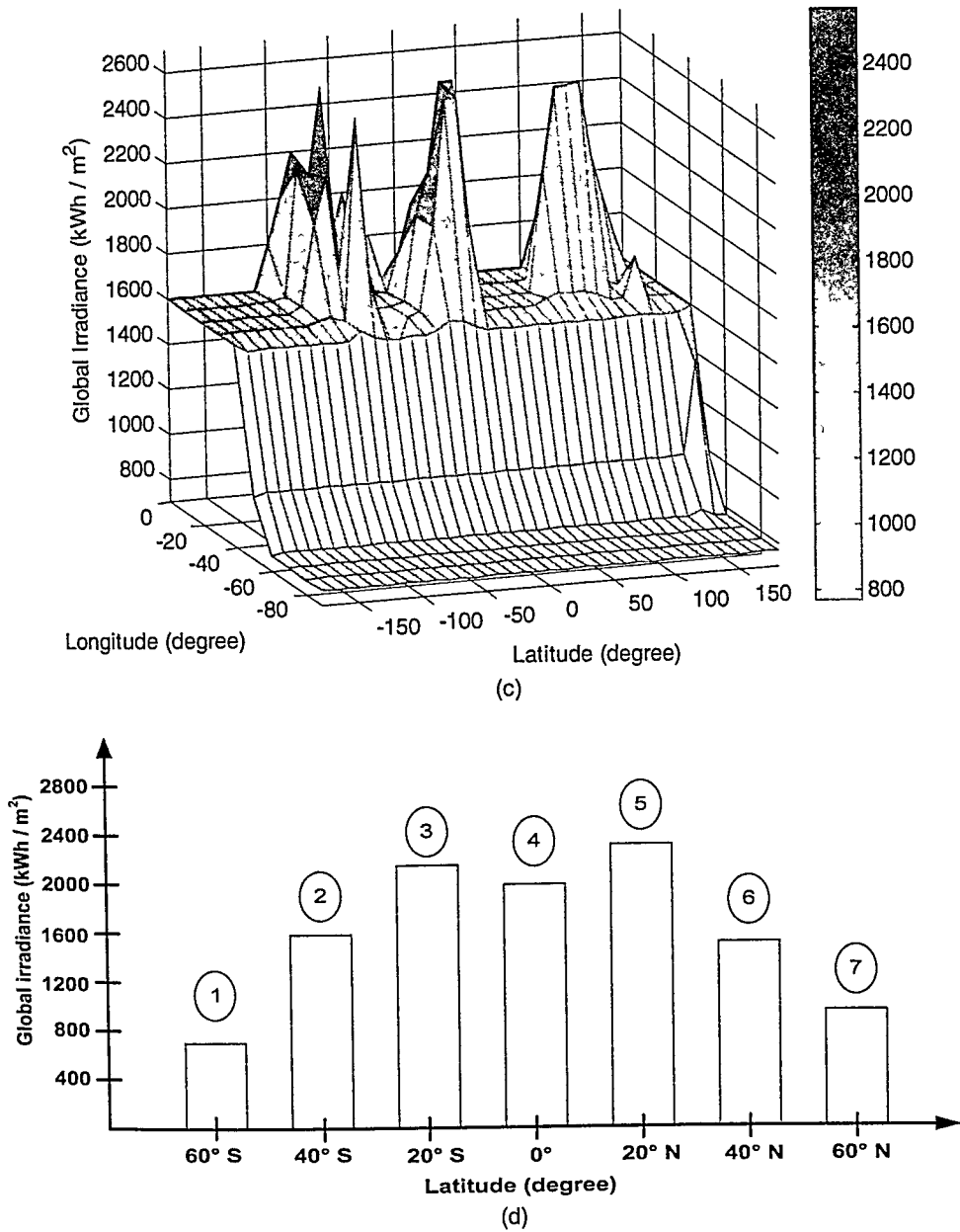
Figure 5.1 (a) The Global Irradiation Values for the World ( \text{kWh}/\text{m}^2 ). 2,3 (b) The Average Northern Hemisphere Global Irradiation Source by Longitude and Latitude. 4,9 (c) The Average Southern Hemisphere Global Irradiation Source by Longitude and Latitude. (d) The Average World Global Irradiation Source by Regions. 4,9 Region 1: Argentina, Chile; Region 2: Argentina, Chile; Region 3: Brazil, South Africa, Peru, Australia, Mozambique; Region 4: Indonesia, Brazil, Nigeria, Columbia, Kenya, Malaysia; Region 5: India, Pakistan, Bangladesh, Mexico, Egypt, Turkey, Iran, Algeria, Iraq, Saudi Arabia; Region 6: China, United States, Japan, Germany, France, United Kingdom, South Korea; Region 7: Russia, Canada, Sweden, Norway.
