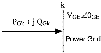
Figure 7.4 A Constant Voltage-Controlled (P-V) Bus.
