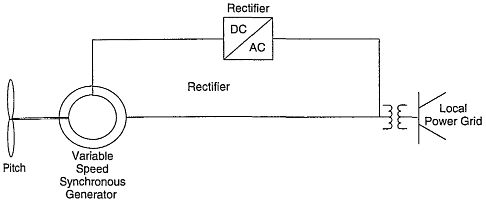
Figure 6.43 A Variable-Speed Synchronous Generator.
