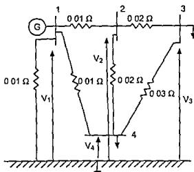
Figure 7.12 The Power Grid for Example 7.3
