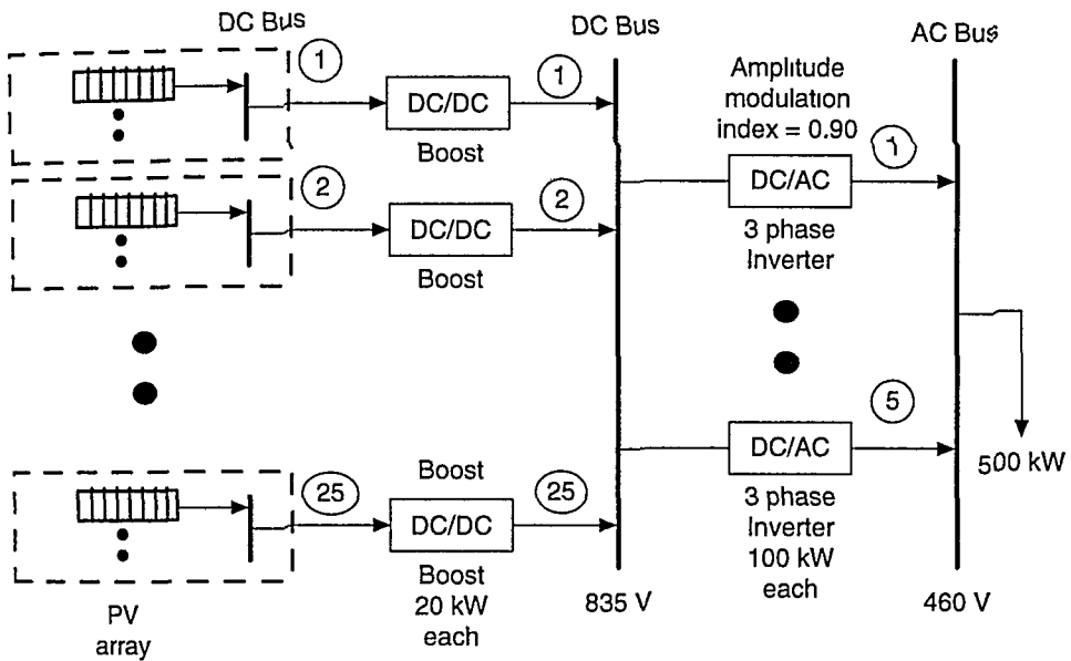
Figure 5.37 The One-Line Diagram of Example 5.6.
