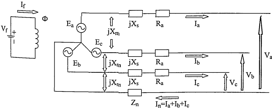
Figure 8.9 A Synchronous Generator Reactance Model.
