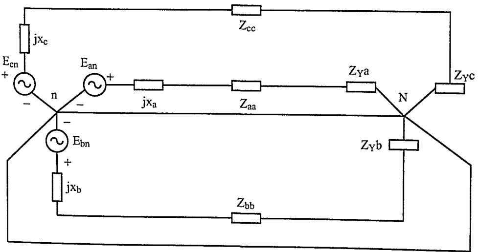
Figure 2.9 The Three-Phase Four-Wire Distribution System.
