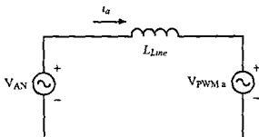
Figure 3.60 The Steady State Per Phase Equivalent Circuit at Steady State for Fundamental Frequency Voltage
