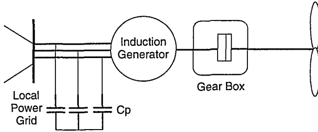
Figure 6.25 A Squirrel Cage Induction Generator with Reactive Power Supplied Locally by a Capacitor Bank.
