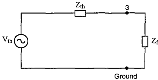
Figure 8.34 The Thevenin Equivalent Circuit for the Fault Current Calculation at Bus 3.
