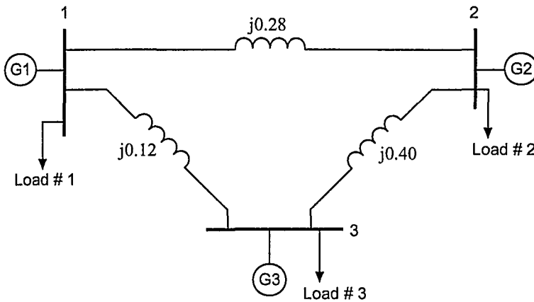
Figure 7.32 The Power Grid for Problem 7.19.
