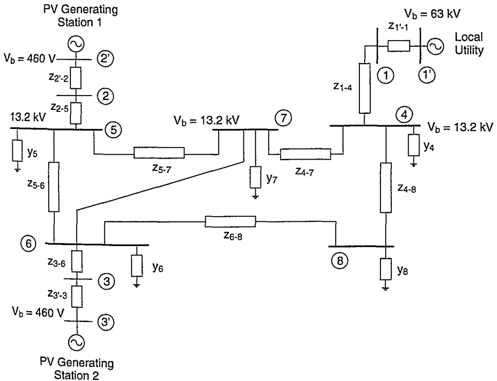
Figure 8.37 Impedance Model for Short-Circuit Studies.
