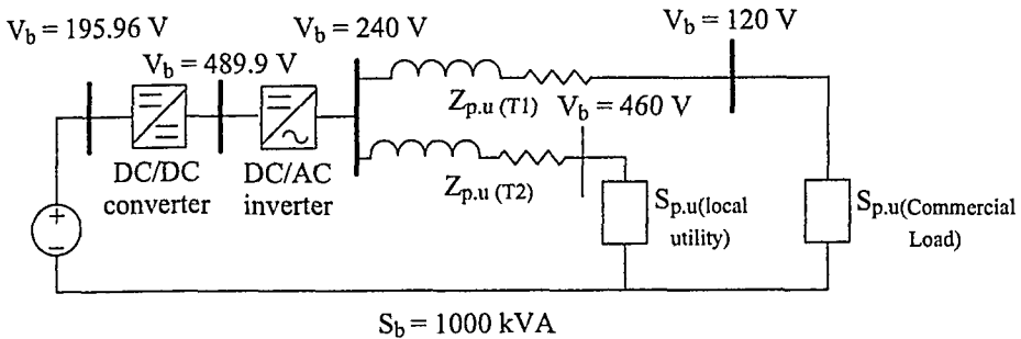
Figure 3.38 The Per Unit Model of Fig. 3.37.
