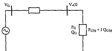
Figure 2.31 The Equivalent Circuit for the Example 2.6
