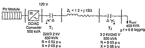
Figure 3.28 The Microgrid of Example 3.8
