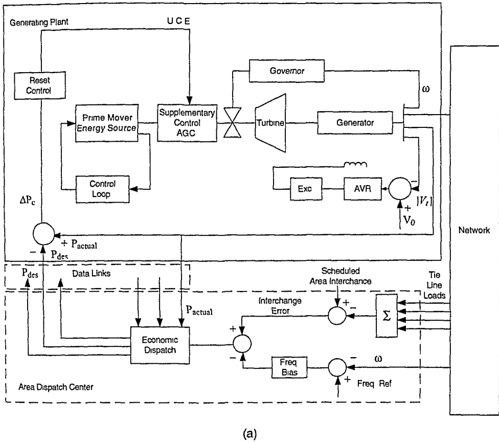
Figure 4.15 (a) Schematic Diagram of Load–Frequency Control System with Economic Dispatch.
