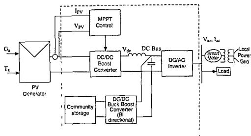
Figure 4.28 A Residential Microgrid Renewable Green Energy (MRG) System with a Local Storage System
