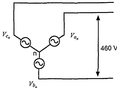
Figure 8.8 The Three-Phase Generator of Example 8.1.
