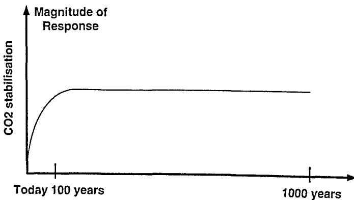
Figure 1.7 \text{CO}_2 Stabilization after \text{CO}_2 Has Been Reduced. (Data from the Intergovernmental Panel on Climate Change, IPCC Third Annual Report. 11 )
