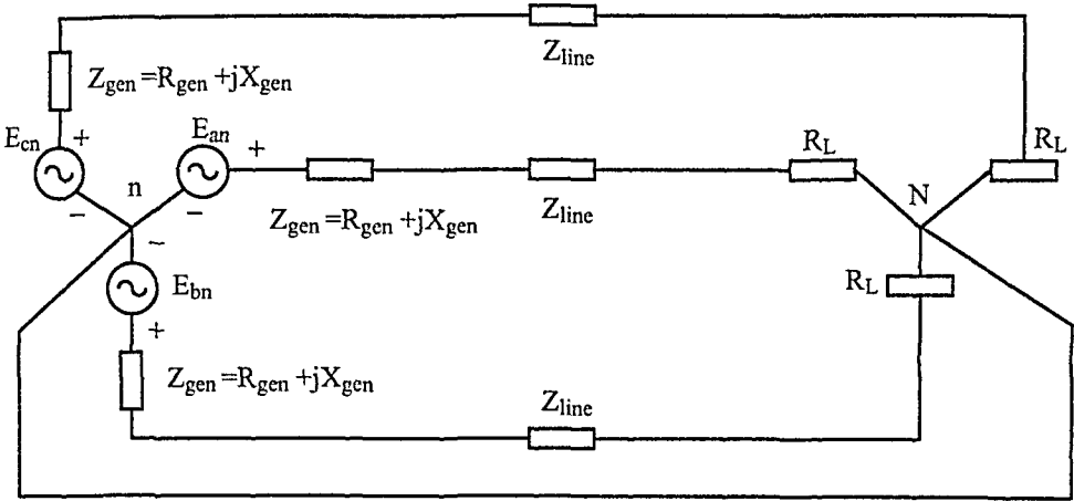
Figure 2.11 A Balanced Three-Phase System.
