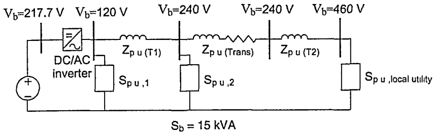
Figure 3.26 Per Unit Model of Fig. 3.25.
