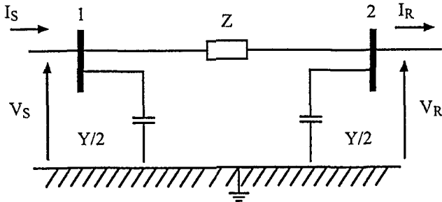
Figure 2.62 A General Model of a Transmission Line.
