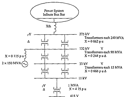
Figure 8.53 A Typical Power Grid System
