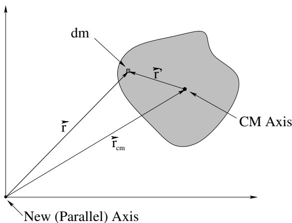
Figure 76: An arbitrary blob of total mass M rotates around the axis at the origin as shown. Note well the geometry of \vec{r}_{cm} , \vec{r}' , and \vec{r} = \vec{r}_{cm} + \vec{r}' .
