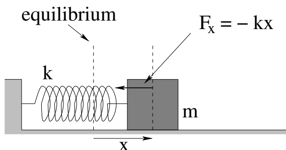
Figure 121: A mass on a spring is displaced by a distance x from its equilibrium position. The spring exerts a force F_x = -kx on the mass (Hooke's Law).
