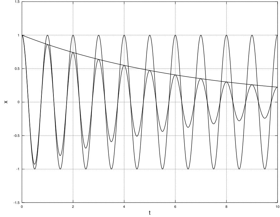
Figure 126: Two identical oscillators, one undamped (with \omega_0 = 2\pi , or if you prefer with an undamped period T_0 = 1 ) and one weakly damped ( b/m = 0.3 ).
