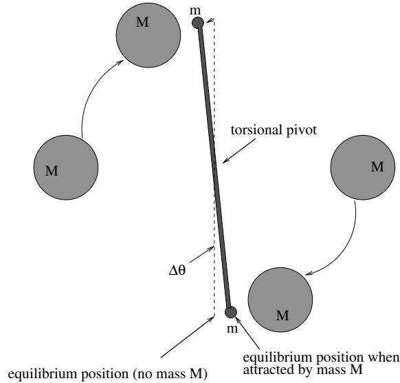
Figure 152: The apparatus associated with the Cavendish experiment , which established the first accurate estimates for G and thereby “weighed the Earth”, the Sun, and many of the other objects we could see in the sky.
