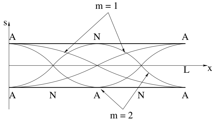
Figure 143: A pipe open at both ends is the exact opposite of a pipe (or string) closed (fixed) at both ends: It has displacement antinodes at the ends. Note well the principle harmonic with a single node in the center. The resonant frequency series for the pipe is the same, however, as for a pipe closed at both ends!
