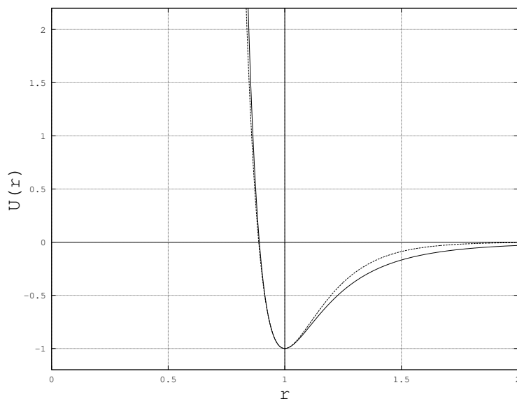
Figure 130: Two “generic” classical potential energy functions associated with atomic bonds on a common scale U_{\min} = -1 , r_b = 1.0 , and a = 6.2 , the latter a value that makes the two potential have roughly the same force constant for small displacements. The solid line is the Lennard-Jones potential U_L(r) and the dashed line is the Morse potential U_M(r) . Note that the two are very closely matched for short range repulsion, but the Morse potential dies off faster than the 1/r^6 London form expected at longer range.
