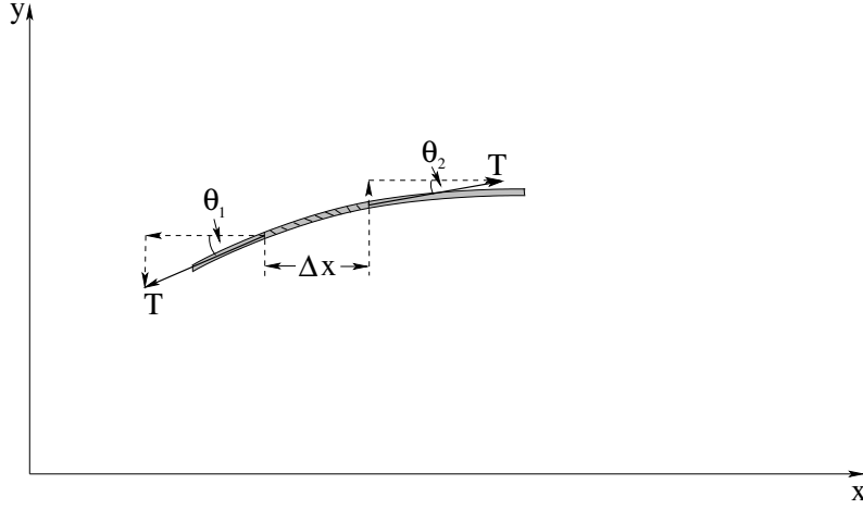
Figure 137: The forces exerted on a small chunk of the string by the tension T in the string. Note that we neglect gravity in this treatment, assuming that it is much too small to bend the stretched string significantly (as is indeed the case, for a taut guitar string).
