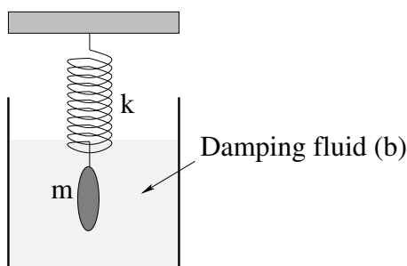
Figure 125: A smooth convex mass on a spring that is immersed in a suitable damping liquid experiences a linear damping force due to viscous interaction with the fluid in laminar flow. This idealizes the forces to where we can solve them and understand semi-quantitatively how to describe damped oscillation.
