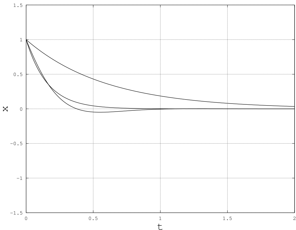
Figure 127: Three curves: Underdamped ( b/m = 2\pi ) barely oscillates. T' is now clearly longer than T_0 . Critically damped ( b/m = 4\pi ) goes exponentially to zero in minimum time. Overdamped ( b/m = 8\pi ) goes to zero exponentially, but much more slowly.
