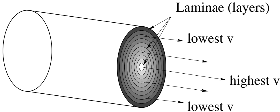
Figure 117: Cross-section of laminar flow in a pipe, where the darker shades correspond to slower-moving fluid in concentric layers (laminae) from the wall of the pipe (slowest speed) to the center (highest speed).
