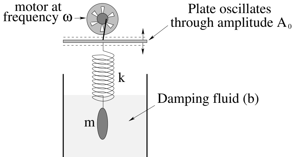
Figure 128: A small frequency-controlled motor drives the “fixed” end of a spring attached to a damped mass up and down through a (variable) amplitude A_0 at (independently adjustable) angular frequency \omega , thereby exerting an additional harmonic driving force on the mass.
