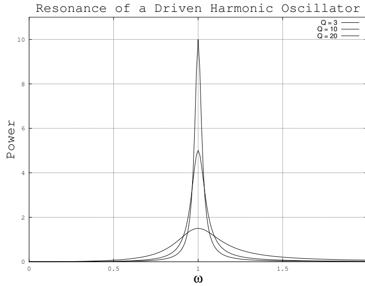
Figure 129: This plots the average power P(\omega) for three resonances. In these figures, F_0 = 1 , k = 1 , m = 1 (so \omega_0 = 1 ) and hence b is the only variable. Since Q = \omega_0/\Delta\omega = m\omega_0/b we plot Q = 3, 10, 20 by selecting b = 0.333, 0.1, 0.05 . Thus P_{\text{max}} = F_0^2/2b = 3/2, 5, 10 respectively (all in suitable units for the quantities involved). Note that the full width of e.g. the Q = 20 curve (with the sharpest/highest peak) is \sim 1/20 at P = P_{\text{max}}/2 = 5 . P is the average power added to the oscillator by the driving force, which in turn in steady state motion must equal the average power lost to dissipative drag forces.
