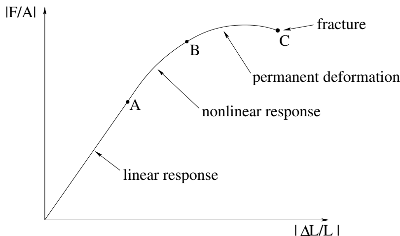
Figure 133: The slope of the linear response part of the curve is Young’s Modulus (note well the absolute magnitude signs). A marks the point where nonlinear response is first apparent. B marks the boundary where dislocations occur and permanent deformation of the material begins. C marks the point where there is a chain reaction – each defect produced produces on average at least one more defect at the same stress, so that the material “instantly” fractures.
