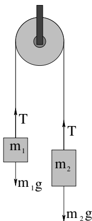
Figure 7: Atwood's Machines consists of a pair of masses (usually of different mass) connected by a string that runs over a pulley as shown. Initially we idealize by considering the pulley to be massless and frictionless, the string to be massless and unstretchable, and ignore drag forces.
