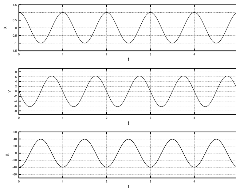
Figure 122: Solutions for a mass on a spring started at x(0) = A = 1 , v(0) = 0 at time t = 0 (so that \phi = 0 ). Note well the location of the period of oscillation , T = 1 on the time axis, one full cycle from the beginning.
