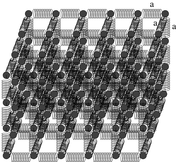
Figure 131: An idealized simple cubic lattice of atoms separated by the “springs” of interatomic forces that hold them in equilibrium positions. The equilibrium separation of the atoms as a .
