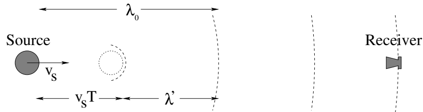
Figure 139: Waves from a source moving towards a stationary receiver have a foreshortened wavelength because the source moves in to the wave it produces. The key to getting the frequency shift is to recognize that the new (shifted) wavelength is \lambda' = \lambda_0 - v_s T where T is the unshifted period of the source.
