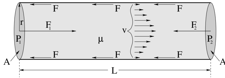
Figure 118: A circular pipe with friction carrying a fluid with a dynamical viscosity \mu – in other words, a “real pipe”. This can be a model for everything from household plumbing to the blood vessels of the human circulatory system, within reason.
