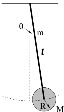
Figure 124: A physical pendulum takes into account the fact that the masses that make up the pendulum have a total moment of inertia about the pivot of the pendulum.
