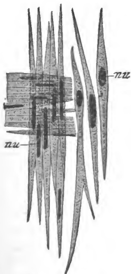
FIG. 14. Unstriated muscle cells from frog's intestine. nu , nucleus. Compare with m.c. in Fig. 19. (From Howes.)
