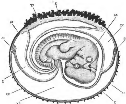
FIG. 154. Rabbit embryo of twelve days' development, with its surrounding membranes, which serve for attachment to the lining of the uterus. (From Marshall.)
