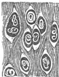
FIG. 109. Trichinae encysted in muscle. (After Leuckart.)
