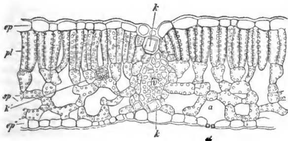
FIG. 30. Cross section of privet leaf. ep , epidermis; pl , palisade cells in upper part of middle tissue; k , deposited crystals; a , air-spaces; v , vascular mid-rib; st , a stoma. (From Strasburger.)
