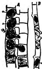
FIG. 77. A, conjugation between cells of two adjacent filaments of Spirogyra . Concentration of protoplasm into one cell of each pair, forming a zygospore (z), is complete in two upper pairs, in progress in next two pairs, and a preparatory stage is beginning in lowest pair of cells. B, conjugation between contiguous cells of the same filament.
