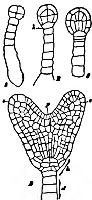
FIG. 62. Stages in development of a seed-plant embryo. The four upper cells in A divide many times (B, C) and form the embryo shown in D with two cotyledons (c), epicotyl (p), and hypocotyl (h). The row of cells shown below the embryo in each figure holds it in position in the ovary. (From Strasburger.)
