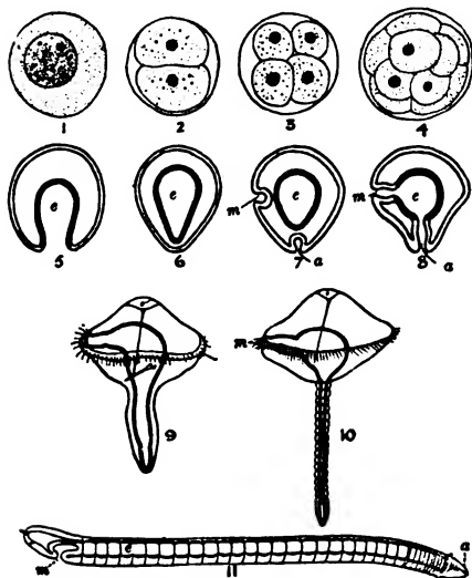
FIG. 111. Development of a marine annelid. 1, fertilized egg-cell; 2, two-cell stage; 3, four-cell stage; 4, eight-cell stage; 5-8, later stages which end in the free-swimming larva, (9), and this metamorphoses (10) into the adult form with numerous segments (11). m , mouth; a , anus; e , alimentary canal. (From Thomson, after Fraipont.)
