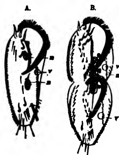
FIG. 89. Division or reproduction of a Stylonichia similar to that of Paramecium . n , nucleus; v , vacuole. (From Hatchesek.)
