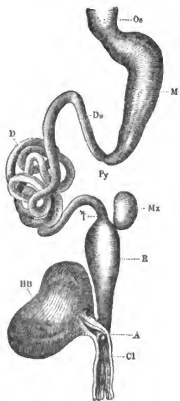
FIG. 8. Alimentary canal of frog. α, esophagus; m, stomach; du, d, small intestine; py, pylorus; mz, spleen; r, large intestine; hb, bladder; cl, cloaca. (From Ecker.)
