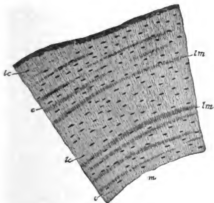
FIG. 13. Cross section of bone from leg of frog. lc , lacunæ or spaces in which lie bone cells; m , marrow cavity in center of leg bone; c , branching tubes from bone spaces and containing branches of the cells; lm , concentric layers of bone deposited by the bone cells. (After Parker and Parker.)
