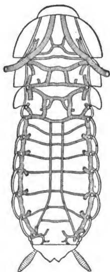
FIG. 132. Arrangement of the larger tubes of the air-tube or tracheal system of a cockroach. (After Miall and Denny.)
