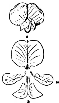
FIG. 31. Pea flower. s, "standard"; w, "wings"; k, "keel"; —see text. (From Gray.)
