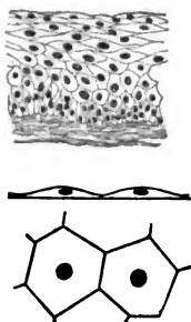
FIG. 10. Upper figure shows that there are many layers of cells in epidermis, those of Fig. 9 being at the surface. The lower diagrams represent two cells in surface and edge views.
