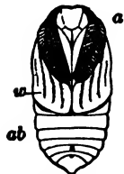
FIG. 134. Pupa of moth. a , antenna case; w , wing case; tongue and leg cases between antennæ; ab , abdomen. (From Kingsley.)
