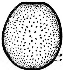
FIG. 44. Transverse section of corn stem showing rind ( r ), pith ( p ), and numerous fibro-vascular bundles ( v ).
