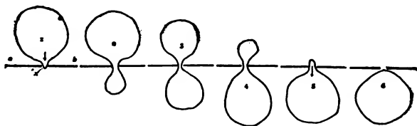
FIG. 92. Diagrams 1-6 show how an amoeba, or a similar white cell from blood of higher animals, passes through very narrow openings.
