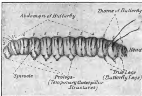
FIG. 133. Butterfly larva. (From Dickerson's "Moths and Butterflies," Ginn & Co.)
