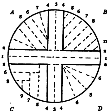
FIG. 56. Four methods of quarter sawing. Cuts 1, 2, 3, 4 remove boards which are perfect radial sections on surfaces 1 and 3. Then each "quarter" is sawed in order 5, 6, 7, 8. The method illustrated in "quarter" C is least desirable.
