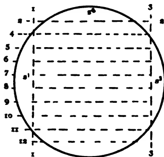
FIG. 55. Ordinary sawing of lumber. s^1, s^2, s^3 , slabs removed by cuts 1, 2, 3; and followed by cuts 4 to 12.
