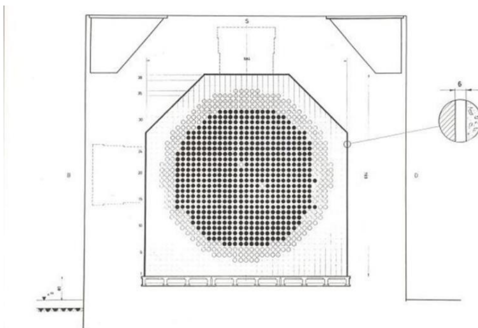
Figure 40: South-North Cross Section of BR1
