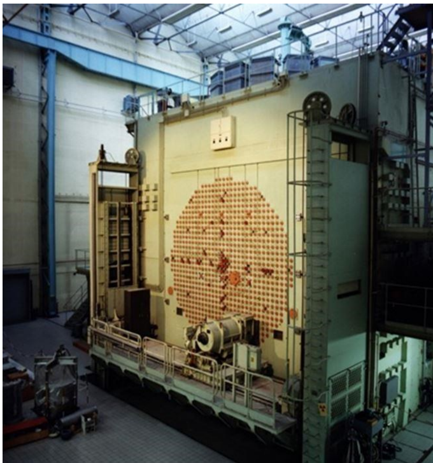
Figure 38: Front view of the BR1 Reactor
