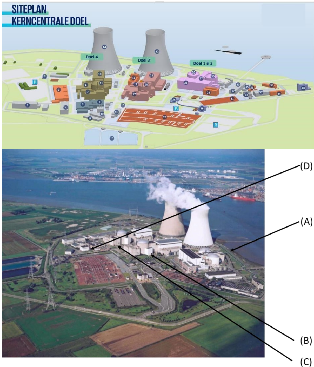
Figure 20: Major buildings of the Doel Site
