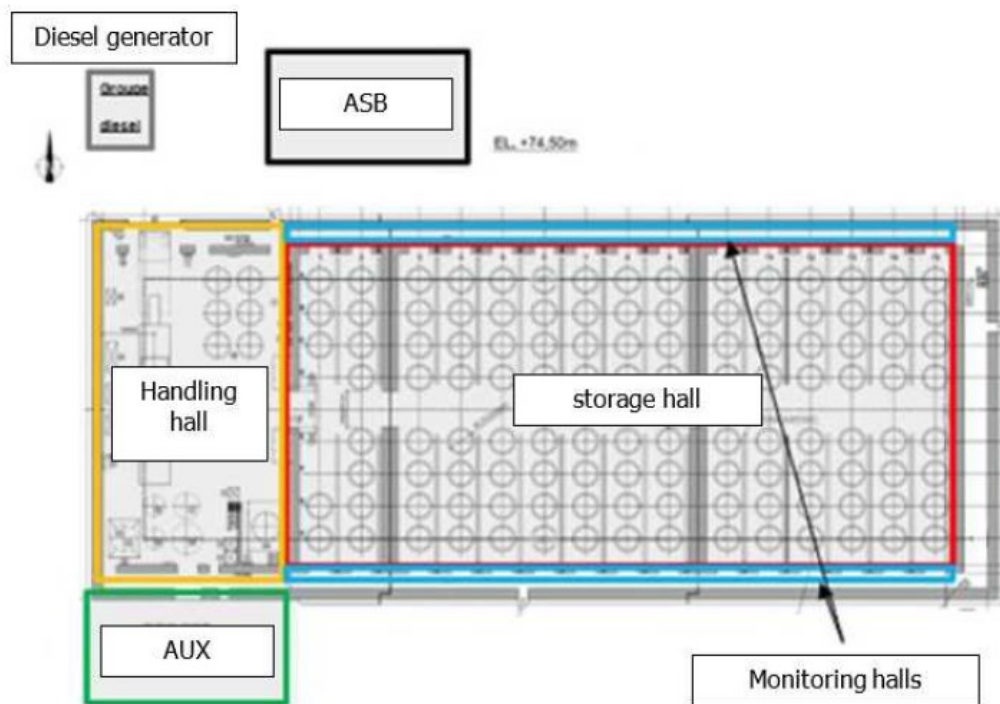
Figure 33: Global layout of the SF 2 facility (illustrated: facility at Tihange site).
