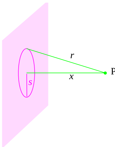
Figure 6.9: Sheet-source geometry.
