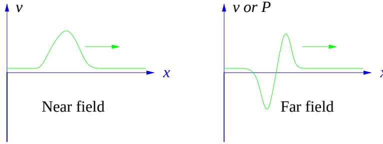
Figure 6.8: Three-dimensional blast wave.
