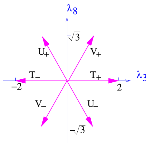
Figure 15.2: The root vectors of \mathfrak{su}(3) .
