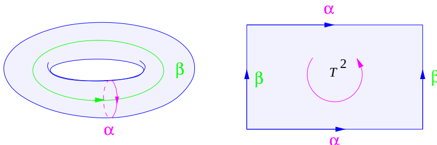
Figure 13.12: Cut-open torus
