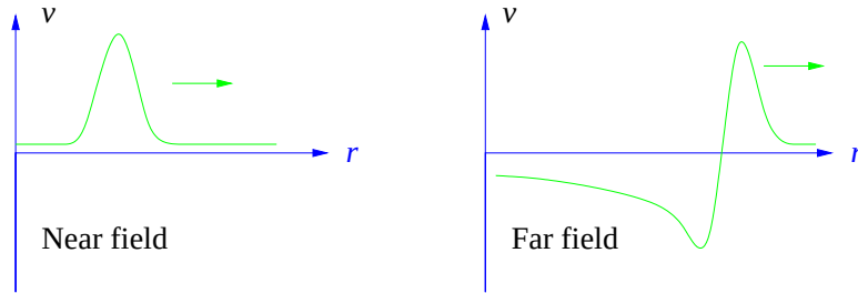
Figure 6.11: In two dimensions the far-field pulse has a long tail.
