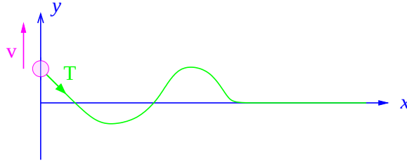
Figure 6.6: A bead connected to a string.
