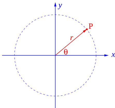
Figure 8.1: Plane polar co-ordinates.
