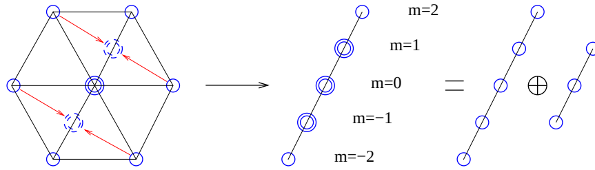
Figure 15.9: The projection and decomposition for 8 = 5 \oplus 3 .
