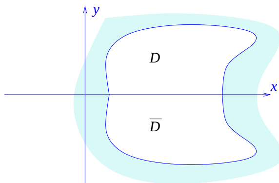
Figure 18.7: The domain D and its mirror image \overline{D} .
