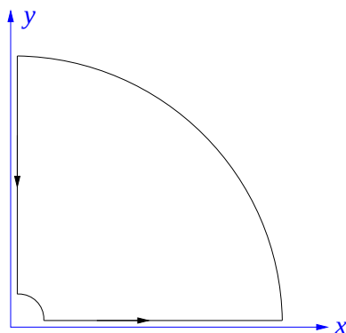
Figure 18.4: Quadrant contour.
