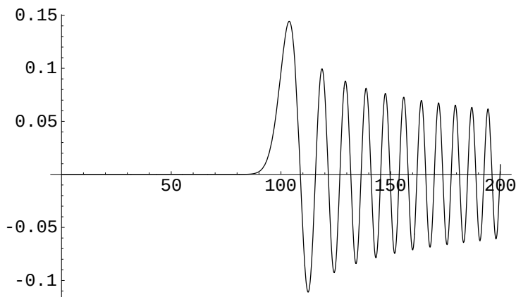
Figure 8.9: J_{100}(x) .
