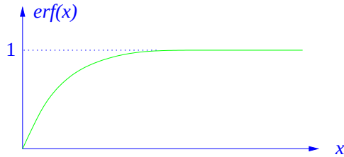
Figure 6.14: Error function.
