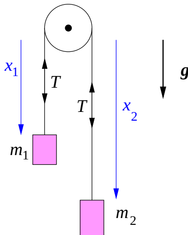
Figure 1.6: Atwood's machine .
