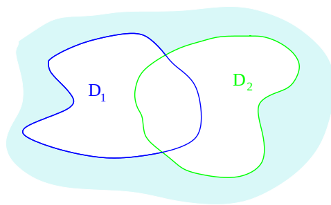
Figure 17.12: Intersecting domains.
