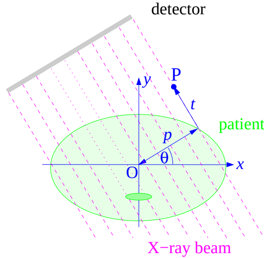
Figure 9.4: The geometry of the CAT scan Radon transformation, showing the location of the point P with co-ordinates x = p \cos \theta - t \sin \theta , y = p \sin \theta + t \cos \theta .
