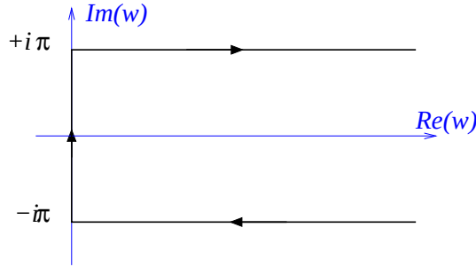
Figure 19.4: Bessel contour after the changes of variables.
