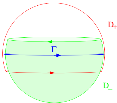
Figure 13.10: A covering the 2-sphere by a pair of contractable caps.
