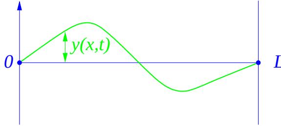
Figure 1.8: Transversely vibrating string
