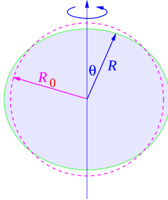
Figure 8.8: Deformed planet.
