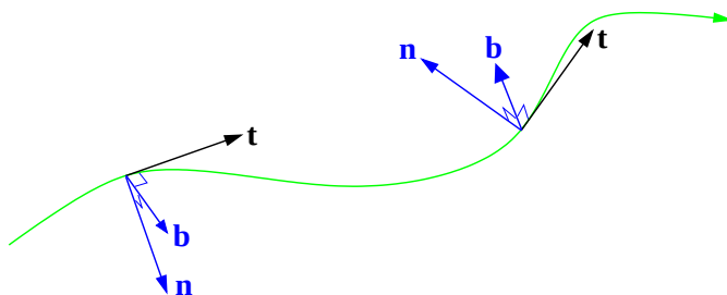
Figure 12.14: Serret-Frenet frames.
