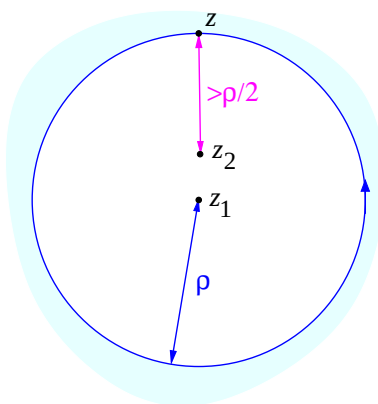
Figure 17.10: Contour for Liouville' theorem.
