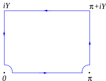
Figure 18.12: Indented rectangle.
