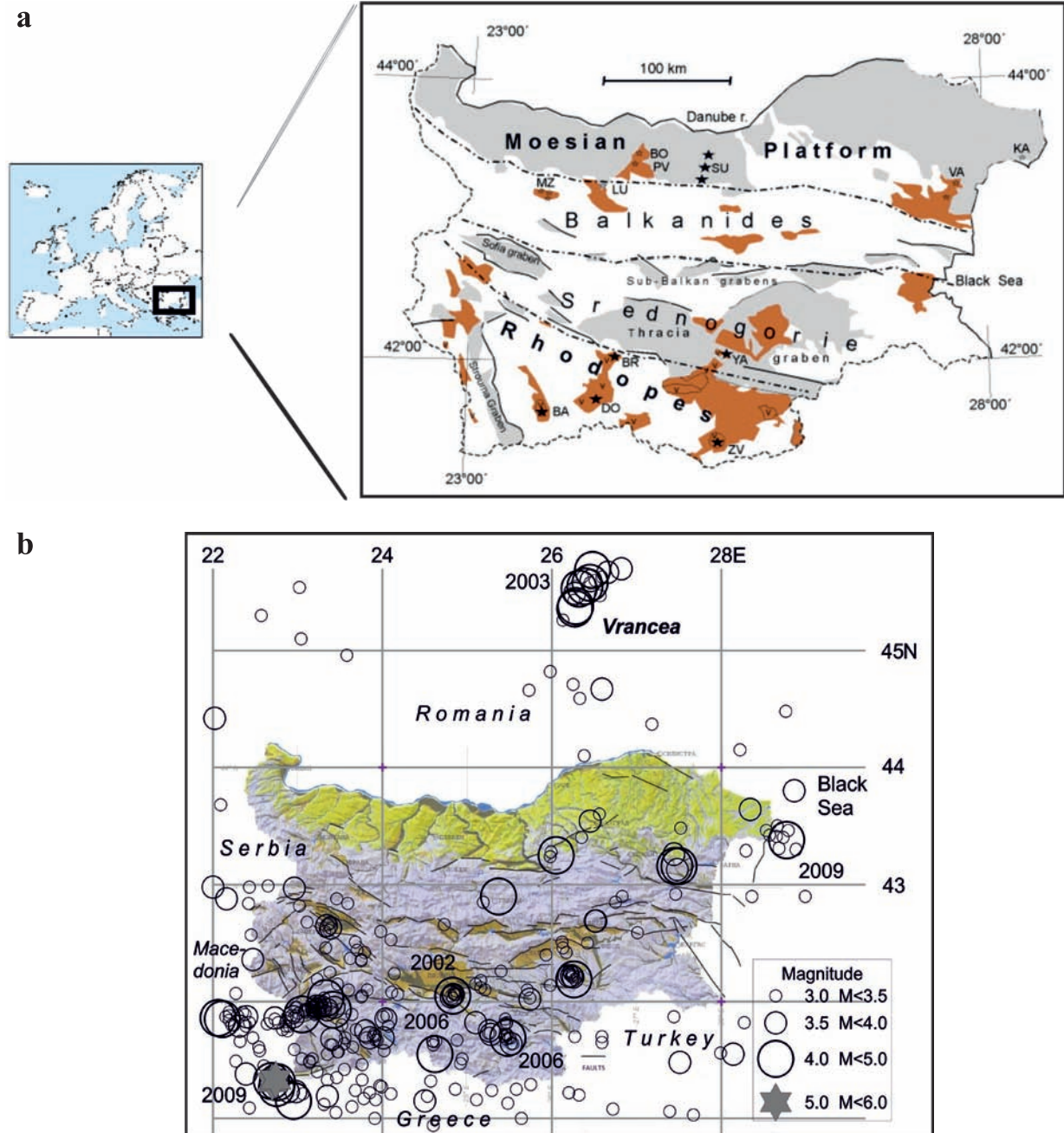
FIGURE 1. a. Main structural and tectonic units in Bulgaria (after van Hinsbergen et al. , 2008), b. Seismicity of Bulgaria (lower magnitude threshold 3.0, time period 2002-2011) on the background of Quaternary faults and Quaternary deposits (< http://www.geology.bas.bg/geotech/Kvaternerni_razlomi.jpg > 2012); the indicated years correspond to earthquakes mentioned in the text (all of them with M > 4 )
